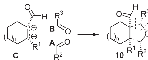
Figure 1. Formation of the bicycles 10 in a highly regio- and stereoselective manner.
