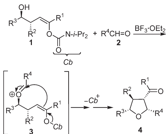
Scheme 1. Synthesis of tetrasubstituted tetrahydrofurans.
