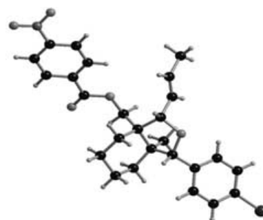
Figure 2. Solid-state structure of 12c . [10]
